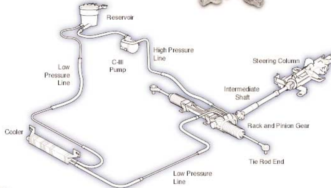
C-III PUMP RESERVOIR 3R700 / 3E764
